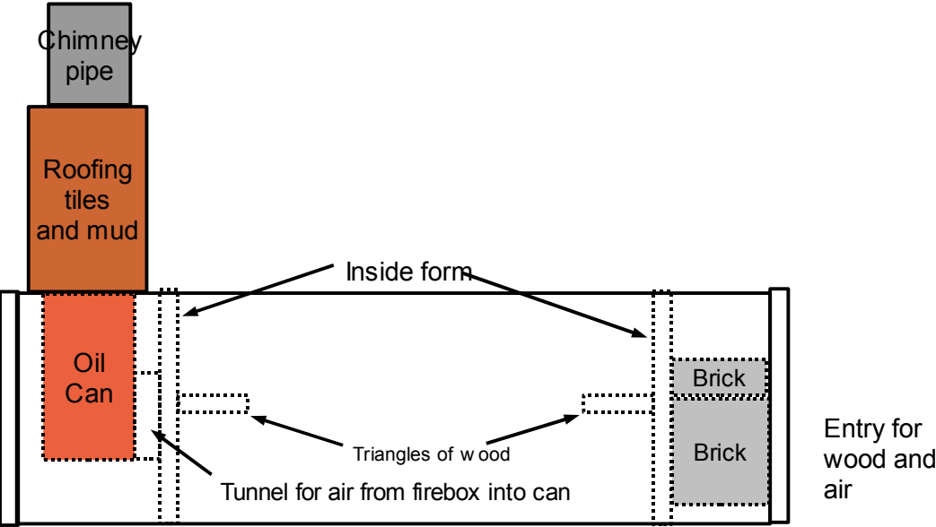
Plan for San Jose Stove – Side View
